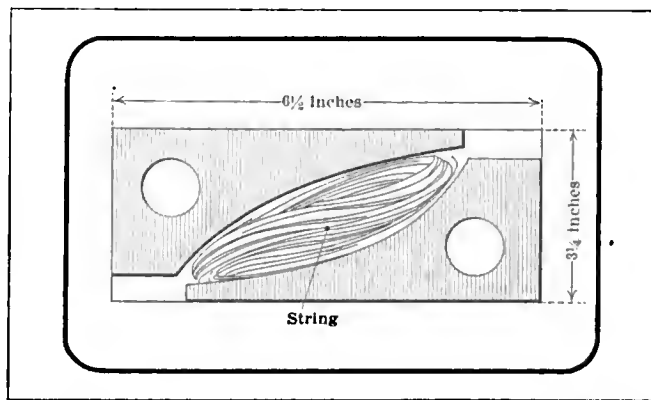
Handy tool-box adjunct—chocks to lock the wheels, and how to carry them
